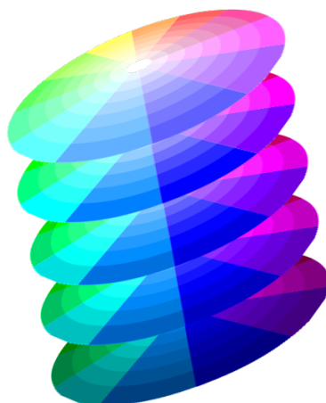
Figure 237: More slices of the HSV representation show how value changes
